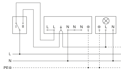
Circuit diagram Connection via a changeover switch for continuous and automatic operation
